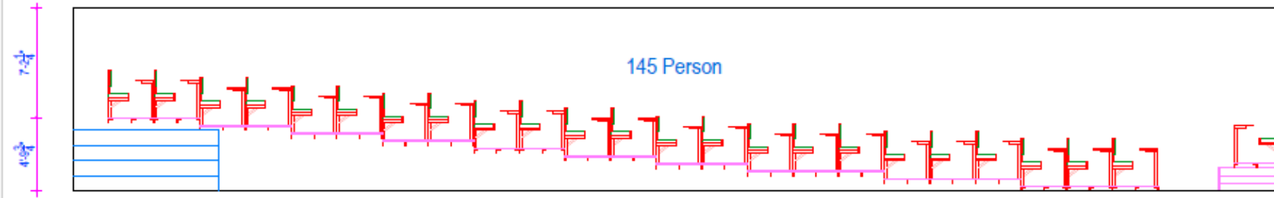
HALL ROOM SECTION
